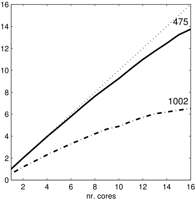
Speedup Sod Shock
