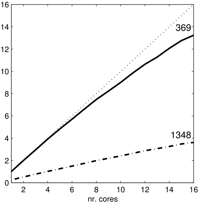
Speedup Sedov Blast
