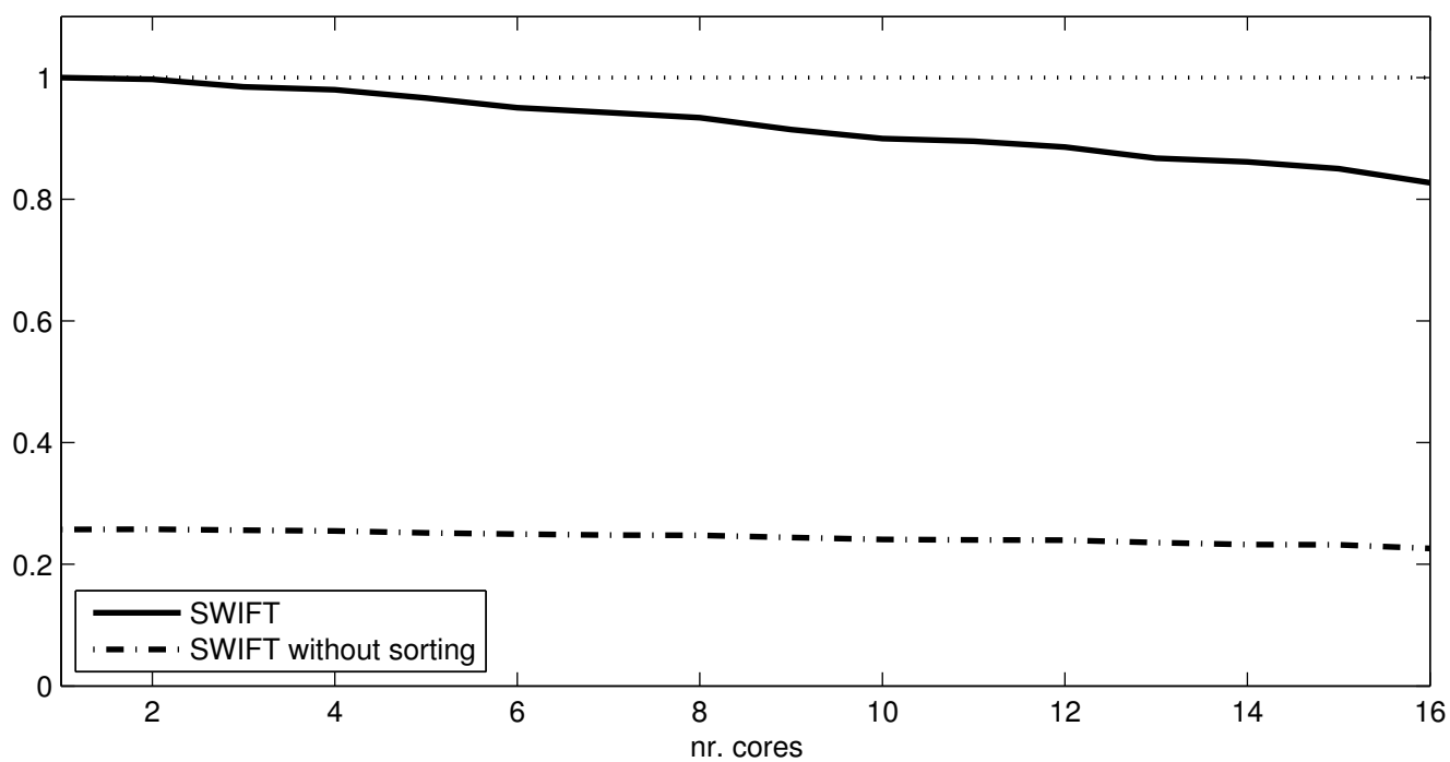
Parallel Efficiency Sedov Blast
