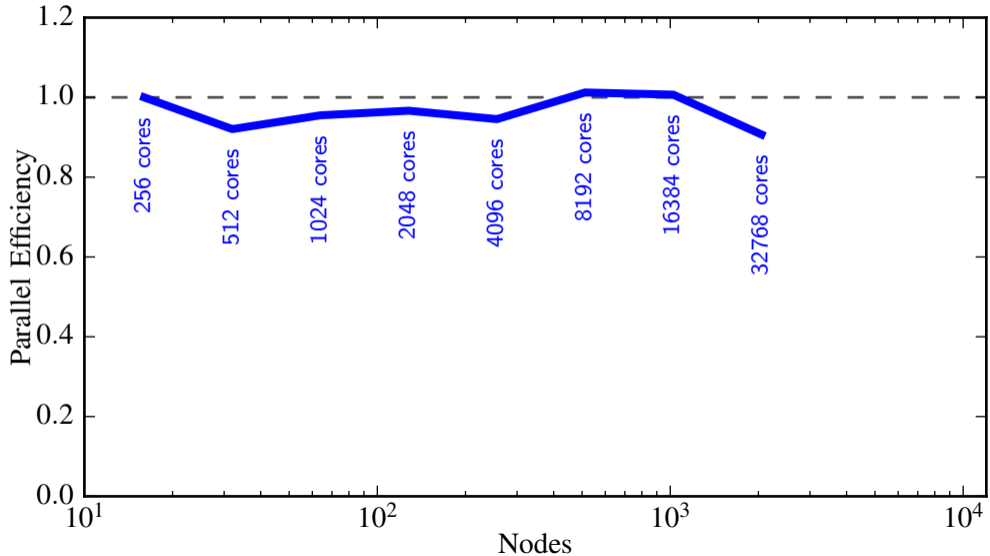
SWIFT Strong scaling on SuperMUC with 512M particles from 16 to 2048 nodes and 16 threads per node
