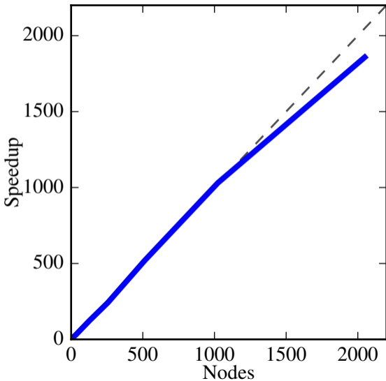
SWIFT Strong scaling on SuperMUC with 512M particles from 16 to 2048 nodes and 16 threads per node
