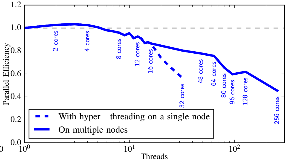
SWIFT Strong scaling on Cosma-5 with 51M particles from 1 to 256 threads
