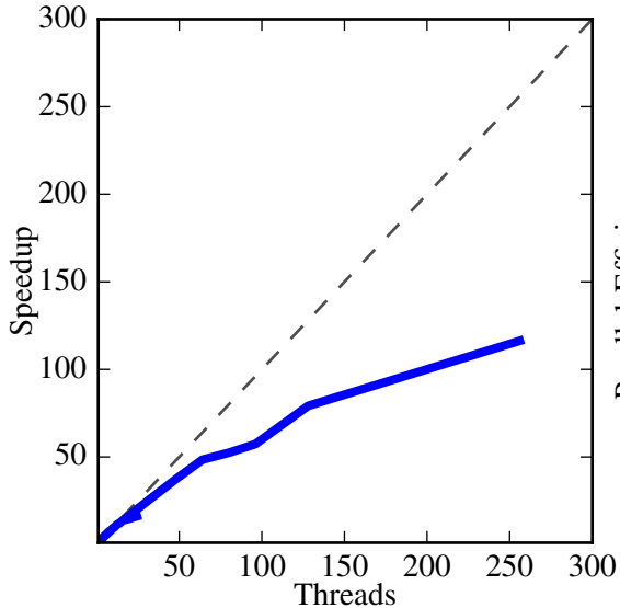
SWIFT Strong scaling on Cosma-5 with 51M particles from 1 to 256 threads
