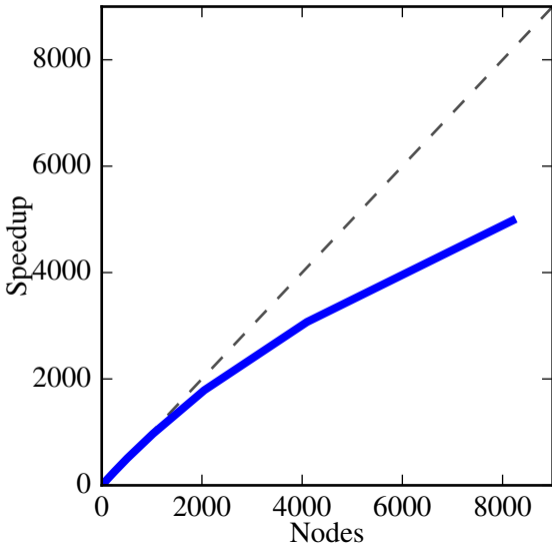
SWIFT Strong scaling on JUQUEEN with 216M particles from 32 to 8192 nodes and 32 threads per node
