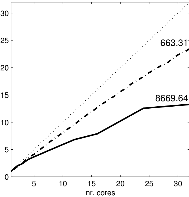
Speedup
