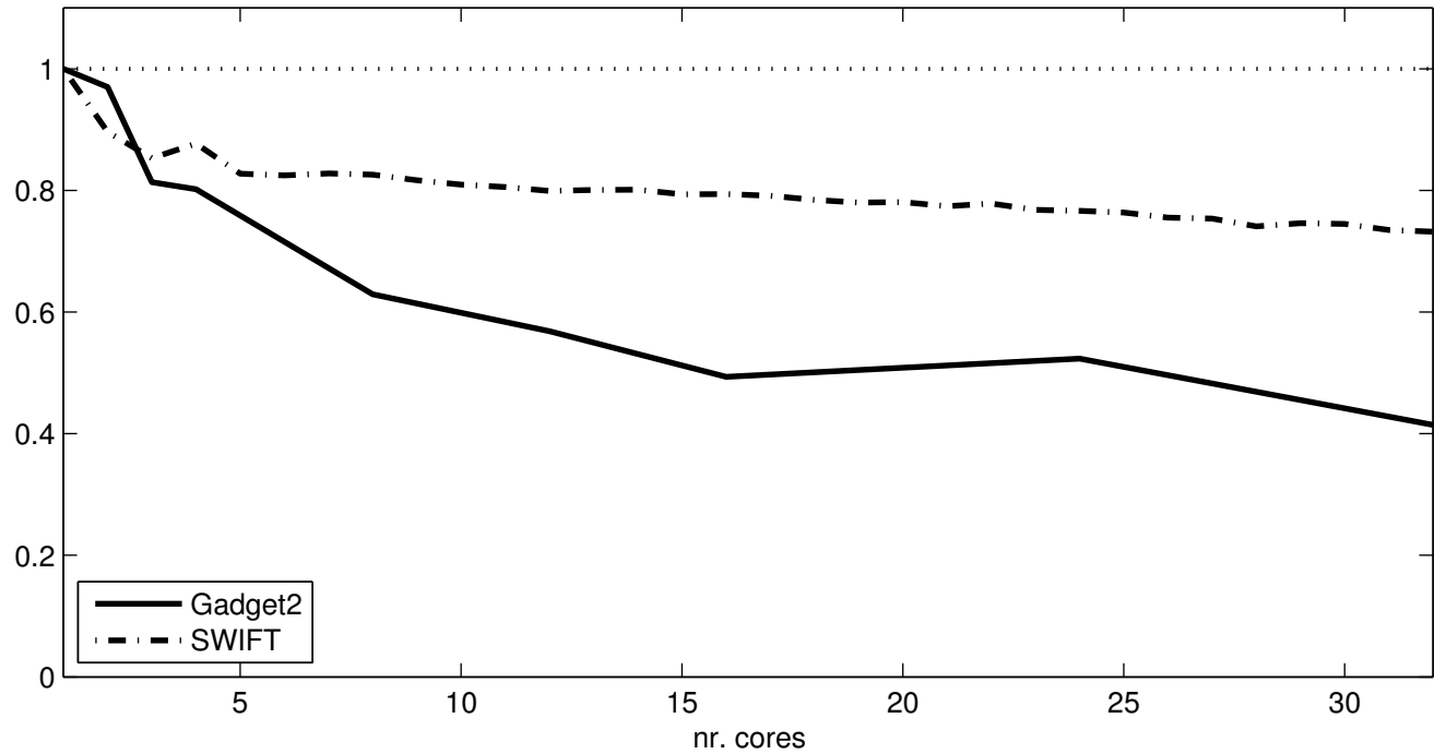
Parallel Efficiency
