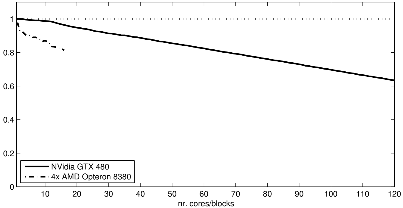
Efficiency JAC
