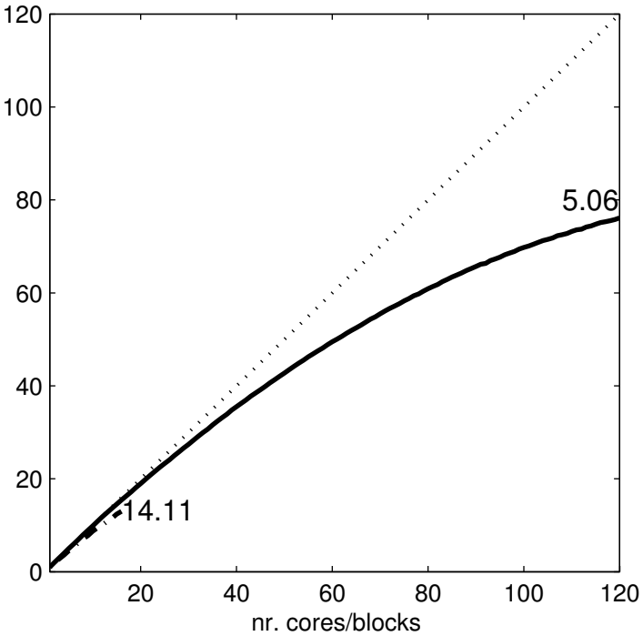
Speedup JAC
