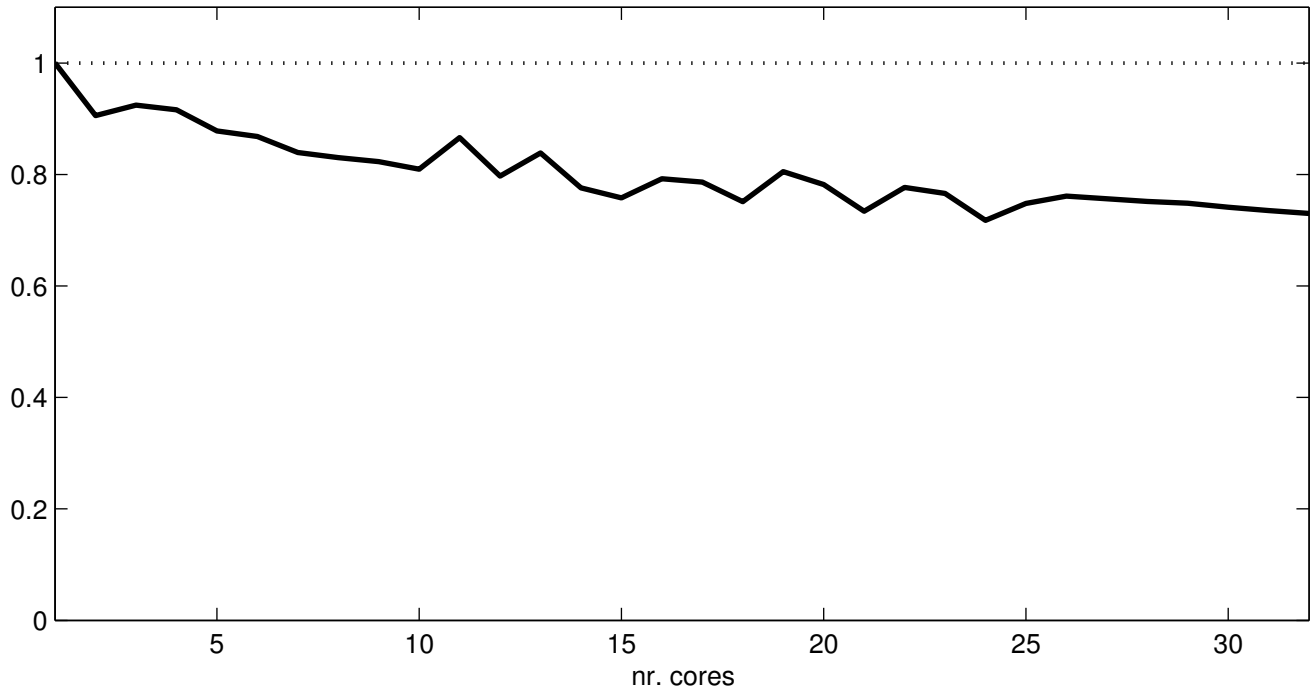
Parallel Efficiency Sod-Shock
