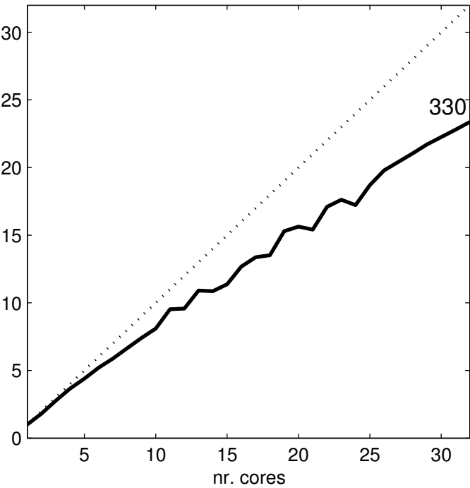
Speedup Sod-Shock
