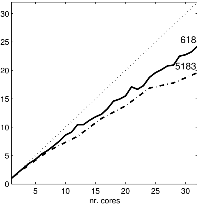
Speedup Cosmological Volume
