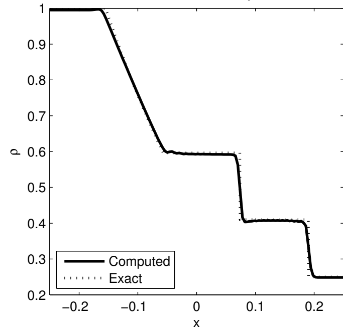
Sod-shock Density
