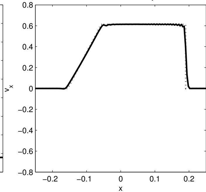
Sod-shock Velocity
