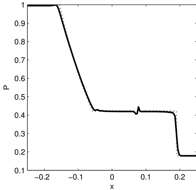
Sod-shock Pressure
