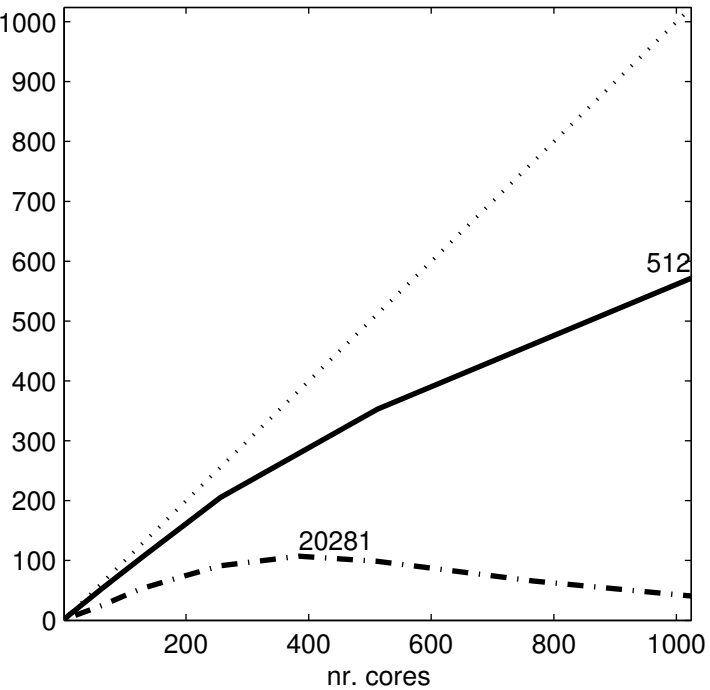
Speedup Cosmological volume
