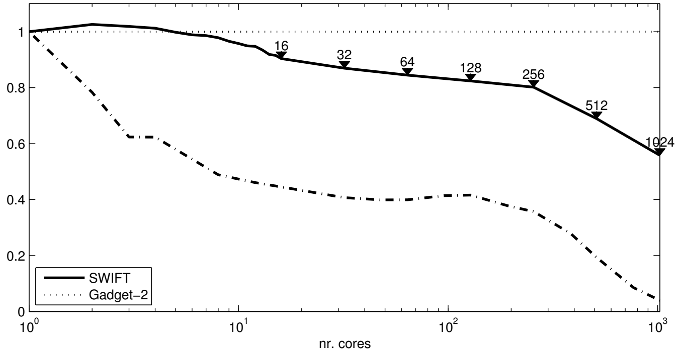
Parallel efficiency Cosmological volume
