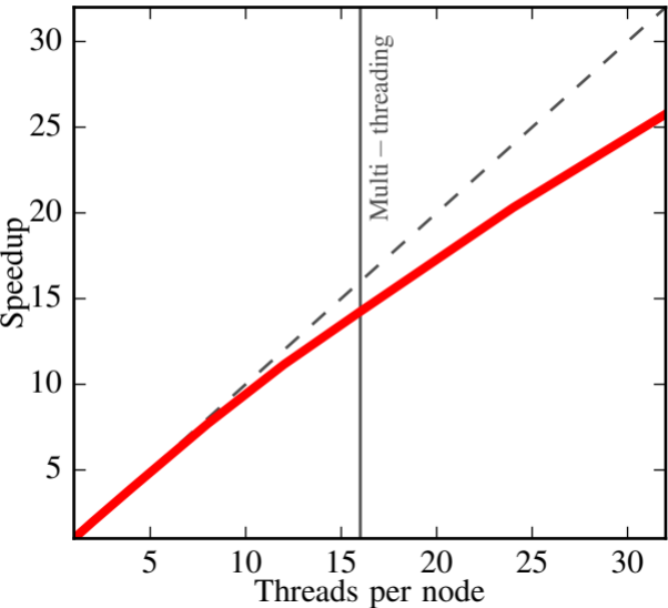
Strong scaling on 512 JUQUEEN nodes
